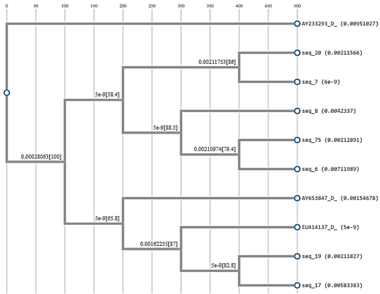
Appendix: Maximum likelihood phylogenetic tree of samples sequenced in this study. Phylogenetic analyses of partial HBV S gene sequences from seven HBV-DNA positive samples revealed that HBV/D was the most prevalent genotype.
